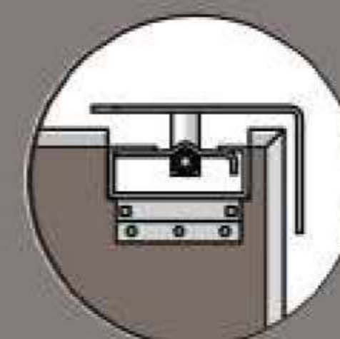
Classic E series gravity close hinge system
