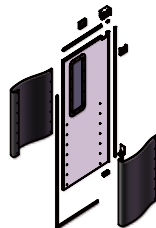
Install gasket bumper and window
